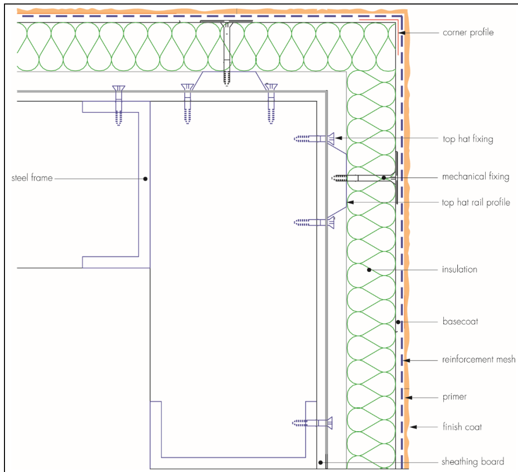
Figure 8 Corner details
