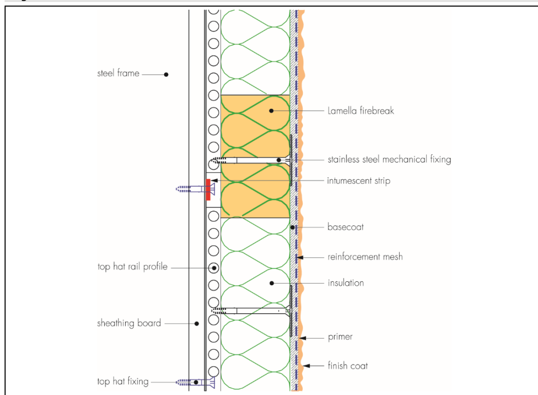
Figure 2 Fire barrier details
