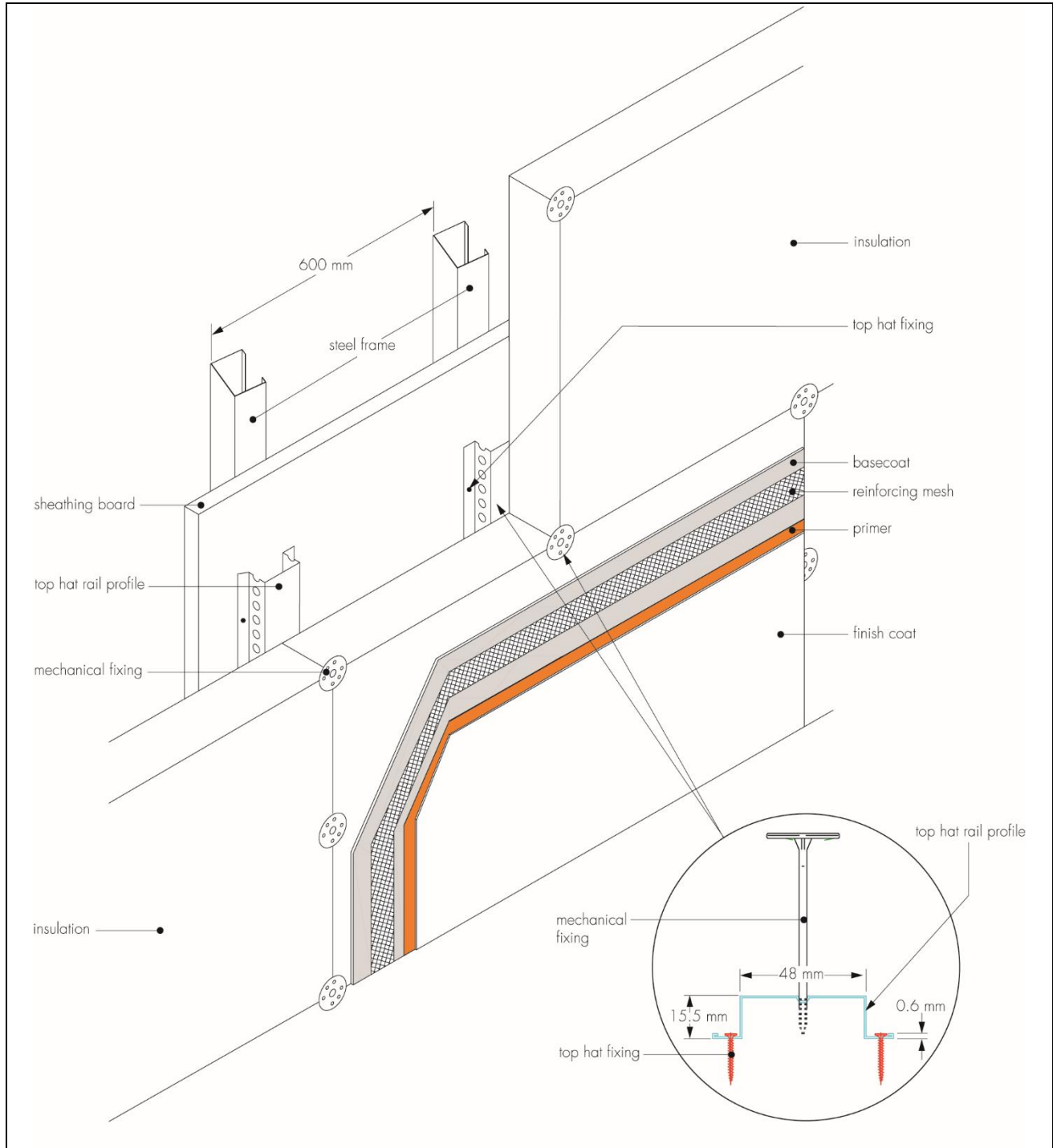
Figure 1 Mapetherm EPS External Wall Insulation System (LWSF)
