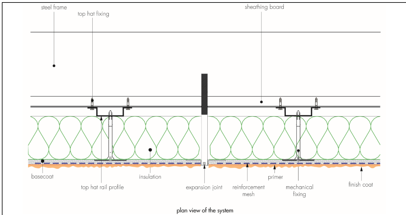
Figure 5 Vertical movement joint
