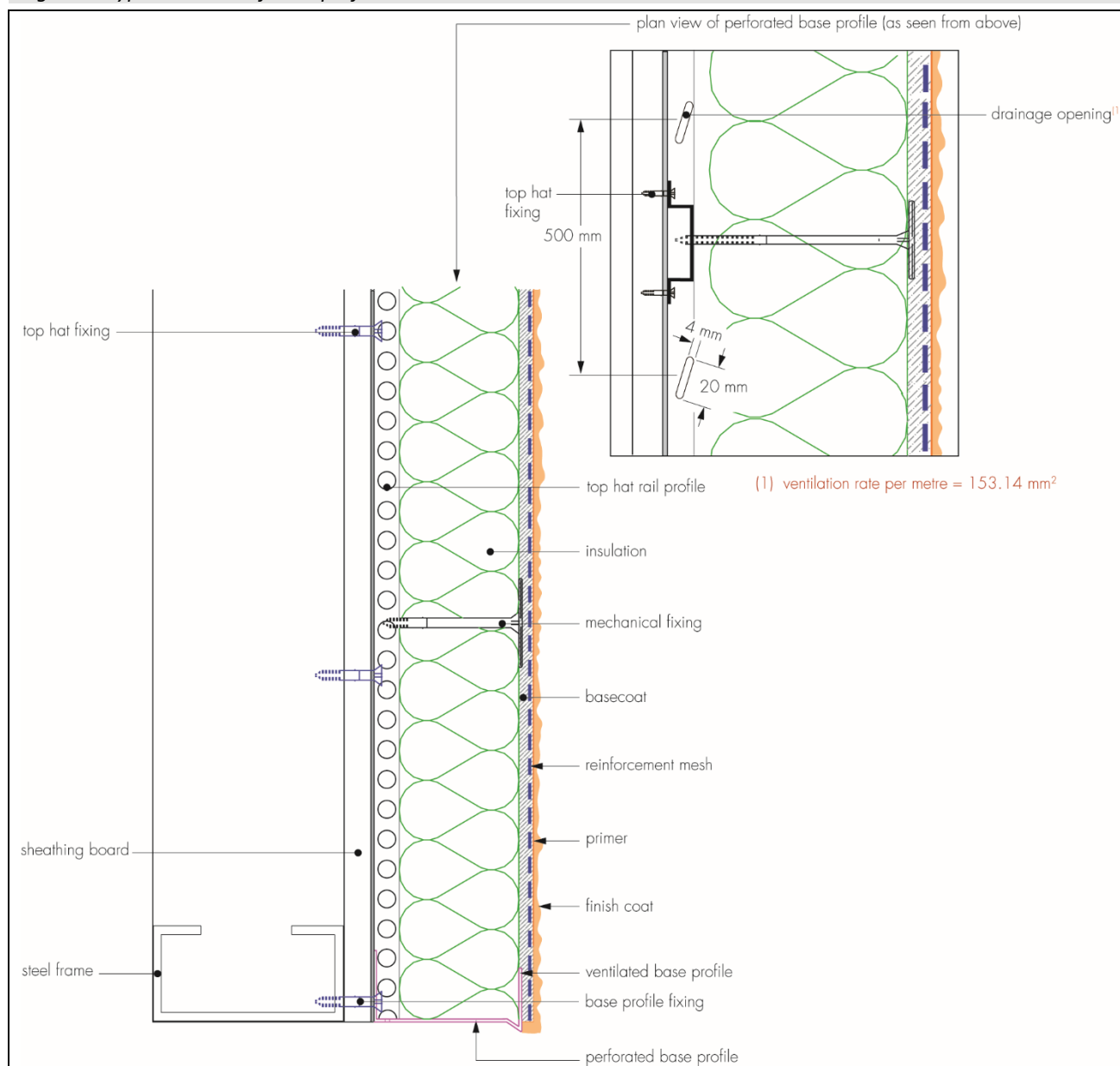
Figure 3 Typical section of base profile
