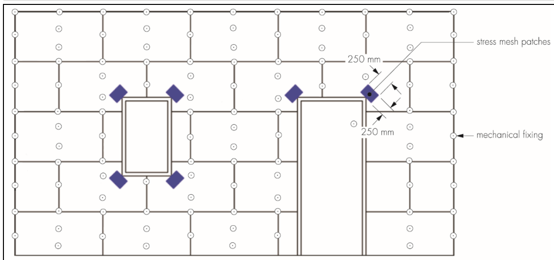
Figure 6 Mechanical fixing pattern and additional reinforcement around openings
