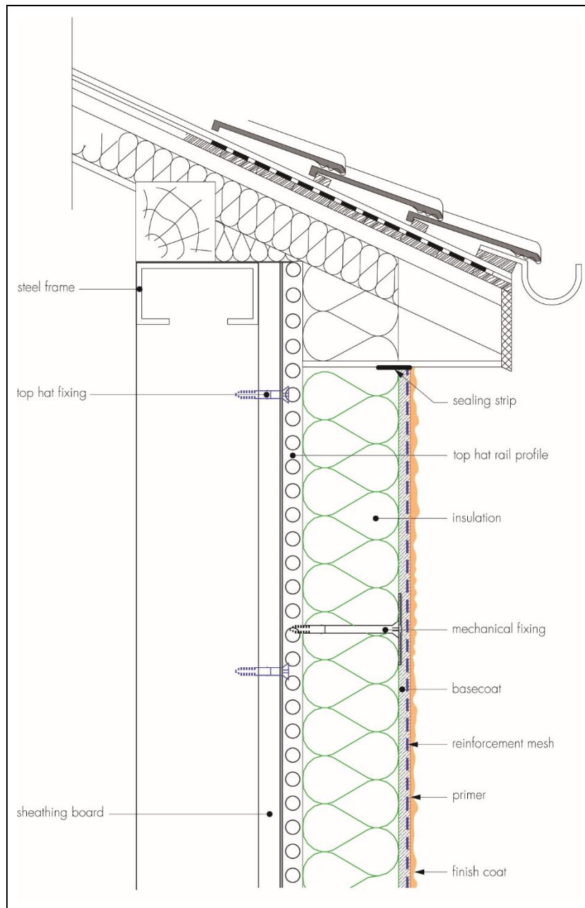
Figure 7 Roof eaves details
