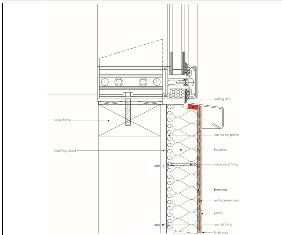
Figure 10 Window sill details
