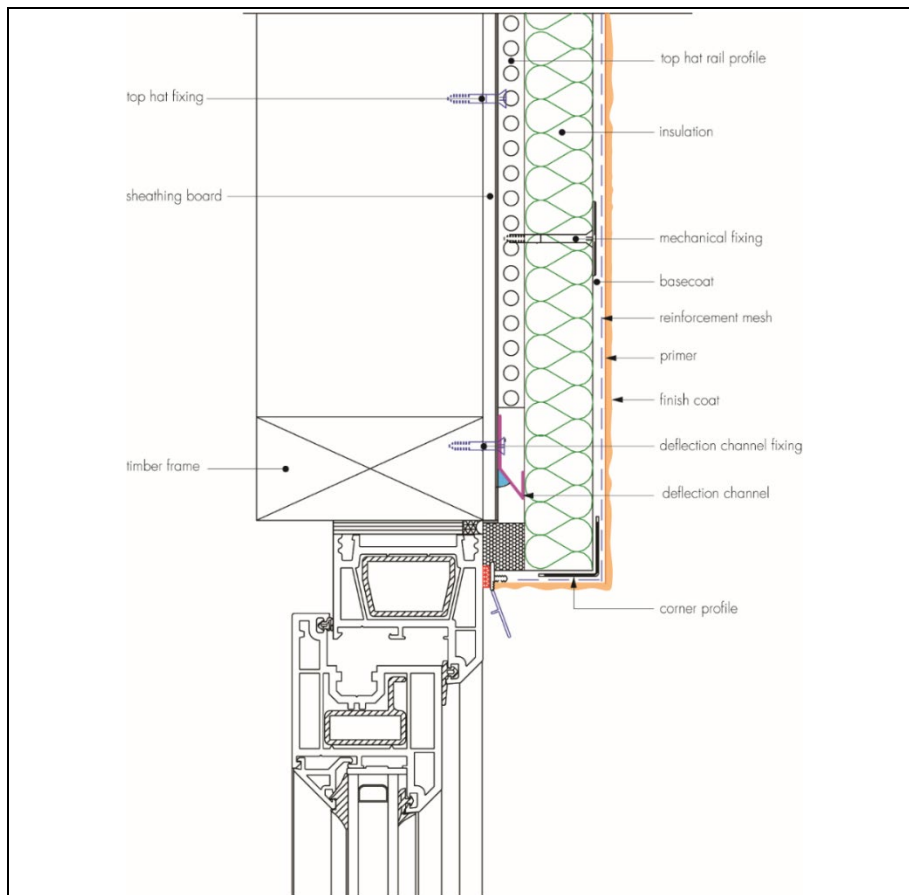
Figure 8 Typical detail at window head details
