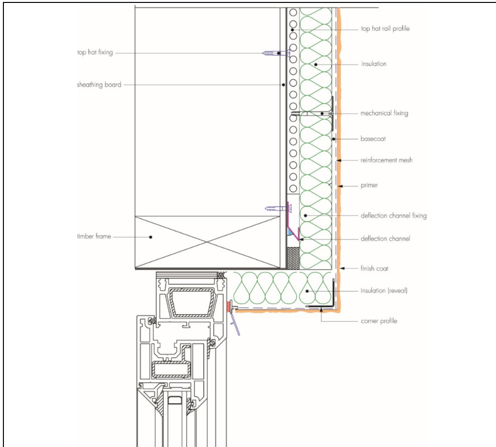
Figure 9 Typical window and door details
