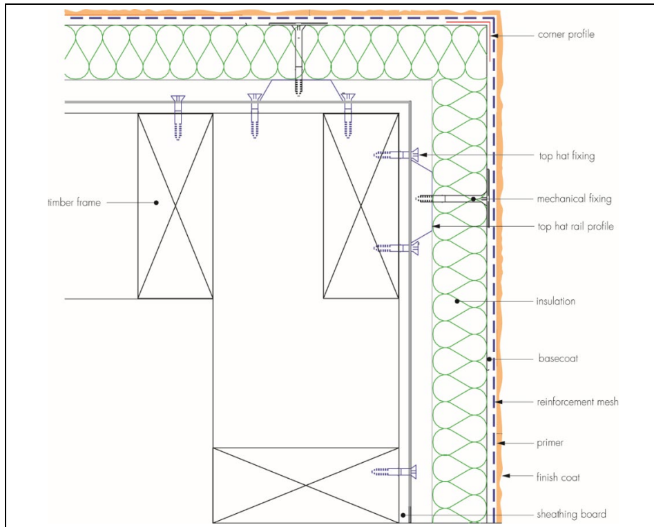
Figure 7 Corner details
