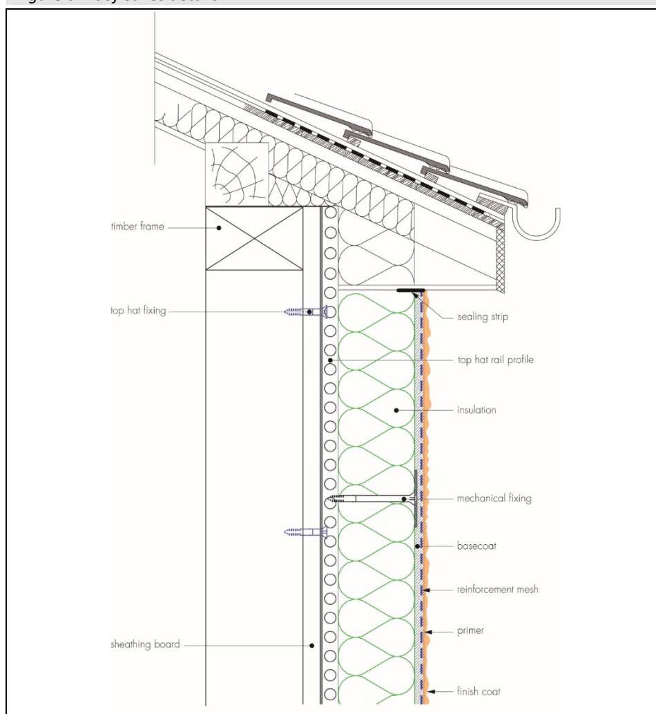
Figure 6 Roof eaves details
