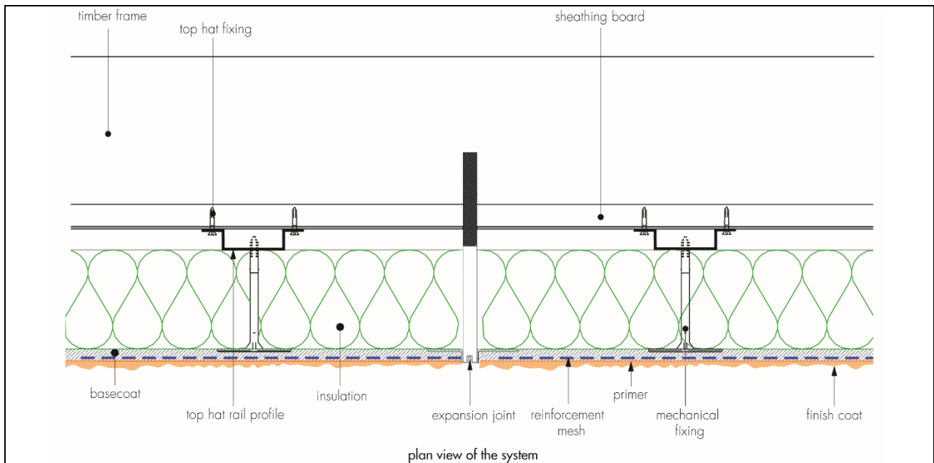
Figure 4 Vertical movement joint
