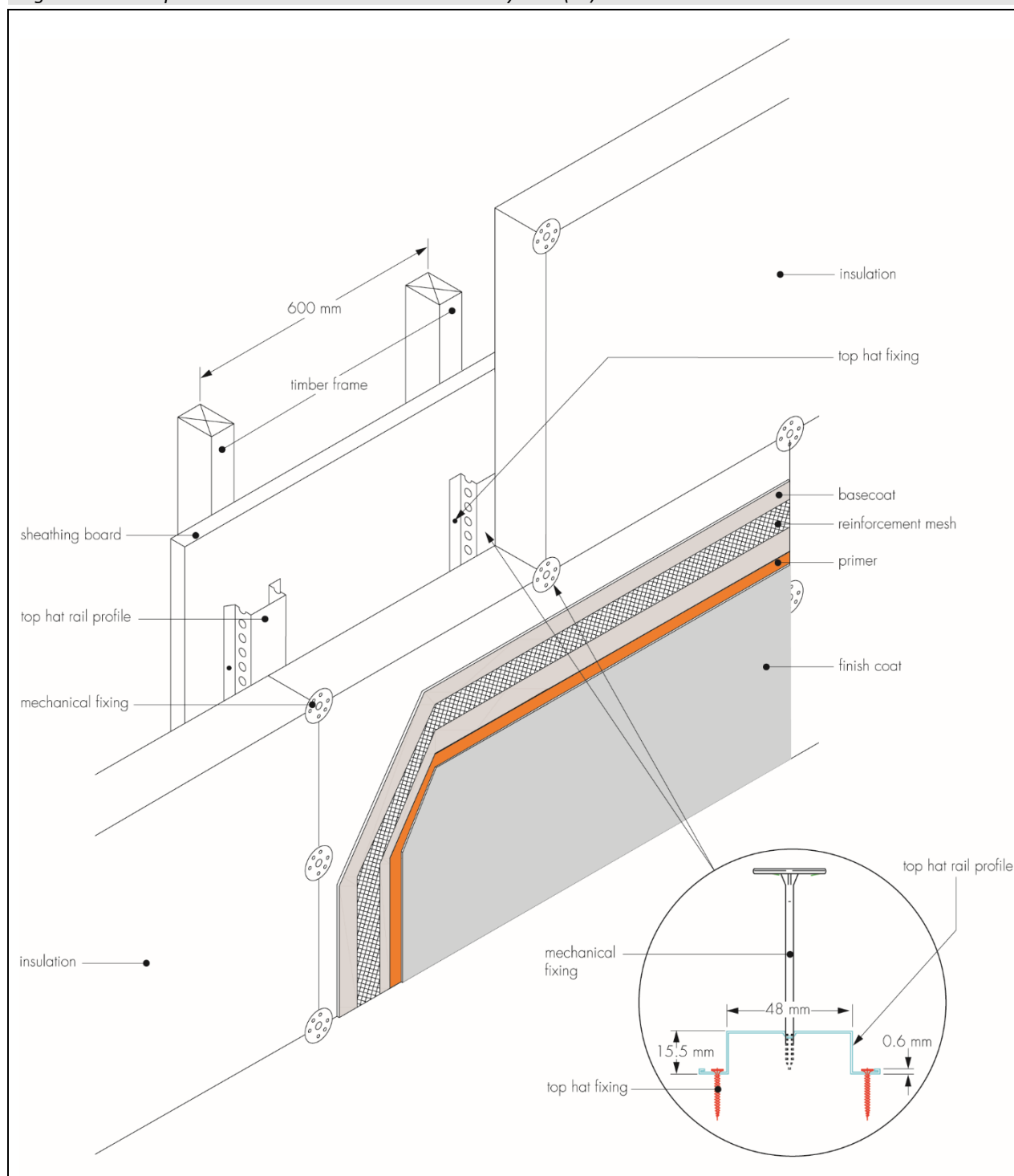
Figure 1 The Mapetherm MW External Wall Insulation System (TF)
