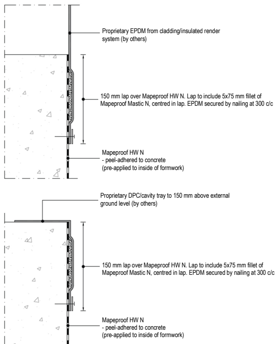
Diagram 1 - Mapeproof HW N - typical termination/continuity details
