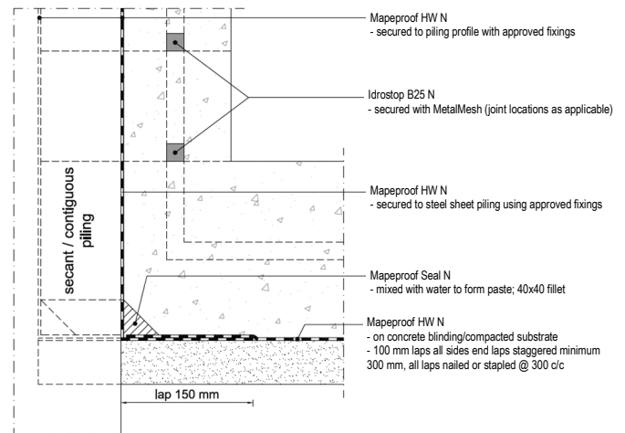
Diagram 2 - Secant/contiguous wall/slab junction
