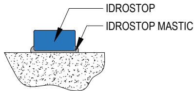
CROSS SECTION OF WATERSTOP
