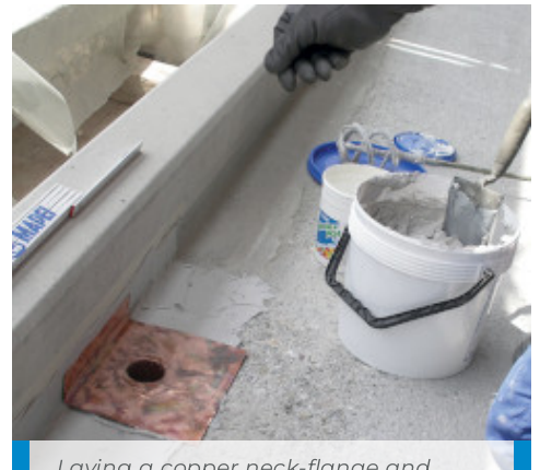
Laying a copper neck-flange and drain spout
