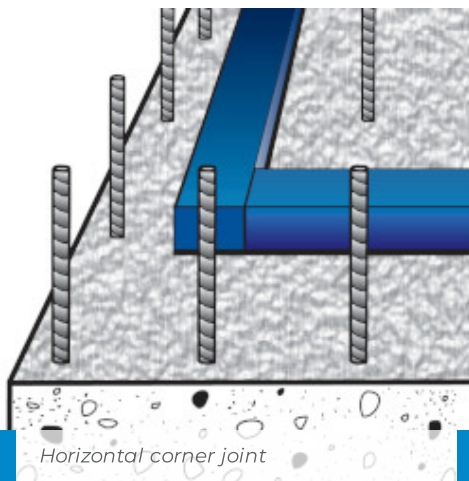
Corner joint between floor and wall
