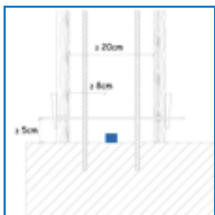
Minimum distance required to obtain the correct confinement of concrete with Idrostop Soft
