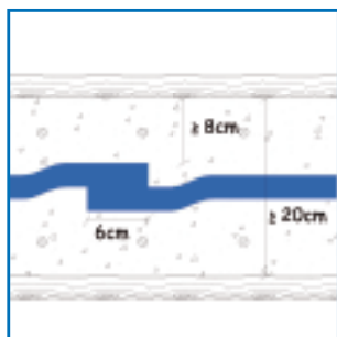
Joint between two pieces of Idrostop Soft butted together lengthways
