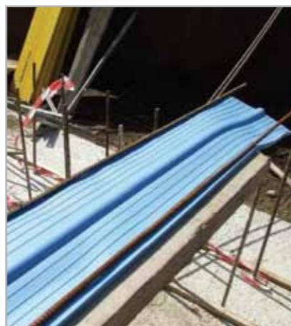
Fig. 7.56a – An example of laying IDROSTOP PVC BI along the centre of a wall when the waterstop has not been clamped in the cast concrete: two lengths of rebar fastened in place with metal wire at the ends of the waterstop
