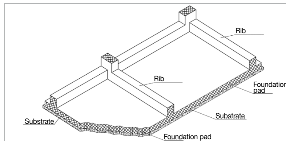
Fig. 2.5 – Ribbed foundation pad
