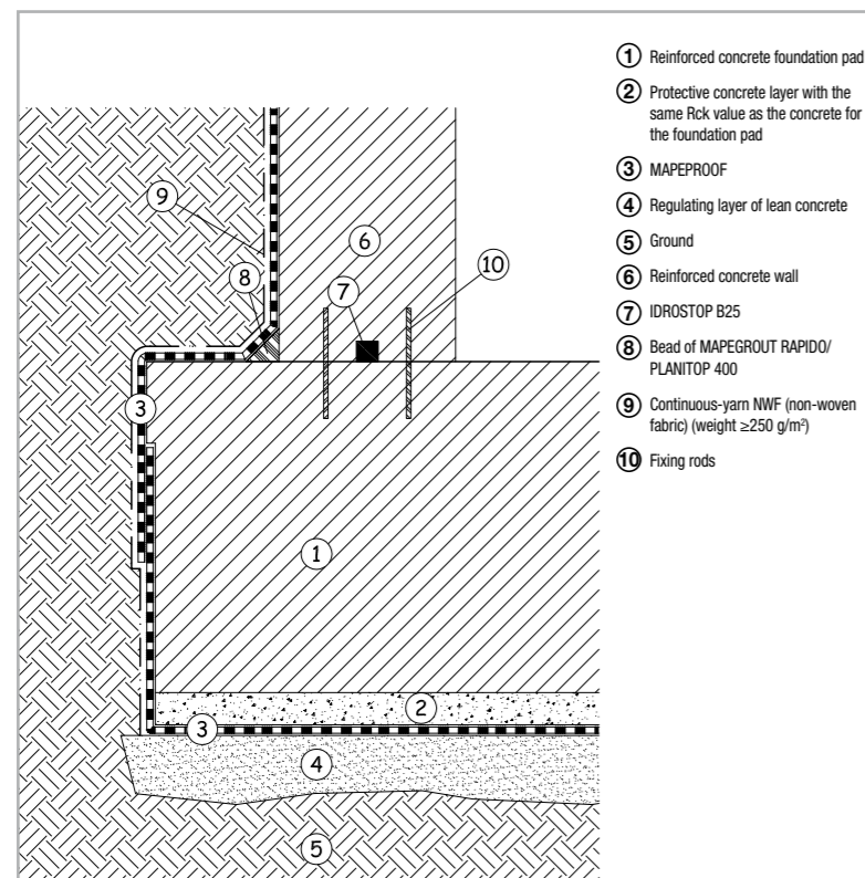
FIG. 7.42 – DETAILED LAYOUT OF WATERPROOFING AFTER CASTING WITH MAPEPROOF
