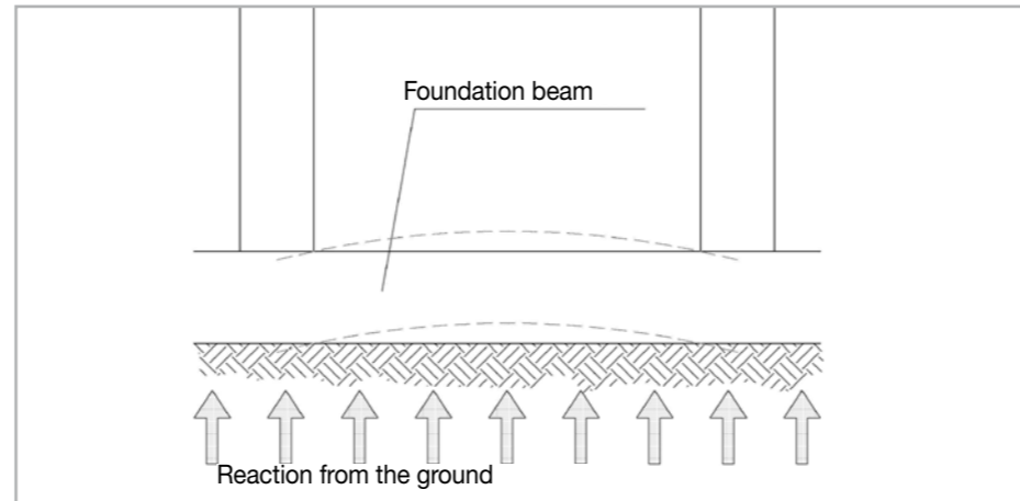
Fig. 2.3 – Schematic diagram of stresses acting on a foundation beam
