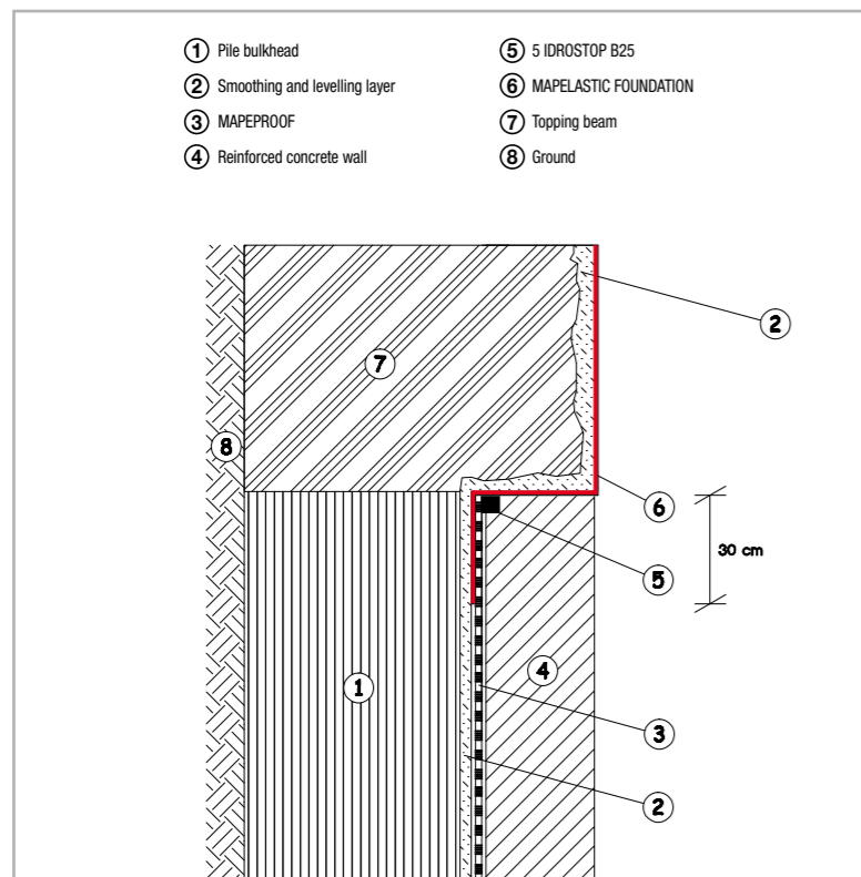
Fig. 7.35 – Waterproofing the topping beam on a bulkhead
