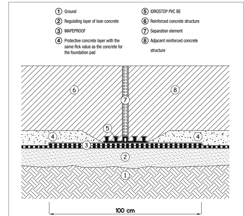
Fig. 7.55 – Detailed layout of sealing a structural joint with IDROSTOP PVC BE
