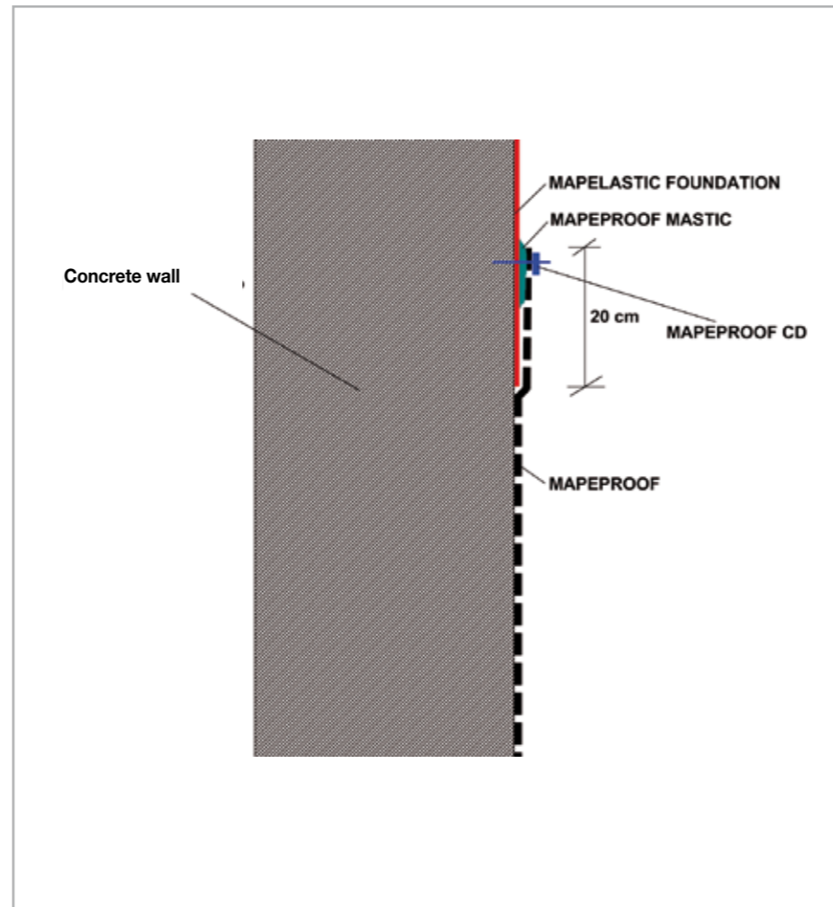
Fig. 7.65 - Schematic layout of sealing a fillet joint between MAPEPROOF and MAPELASTIC FOUNDATION using MAPEPROOF MASTIC
