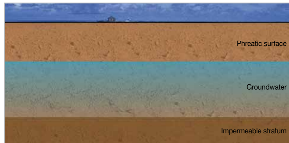
Fig. 3.2 - Sectional view of a portion of ground and its water table
