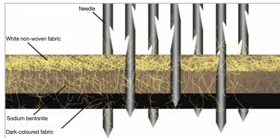
Fig. 5.2 – A schematic view of the needle-punch process
