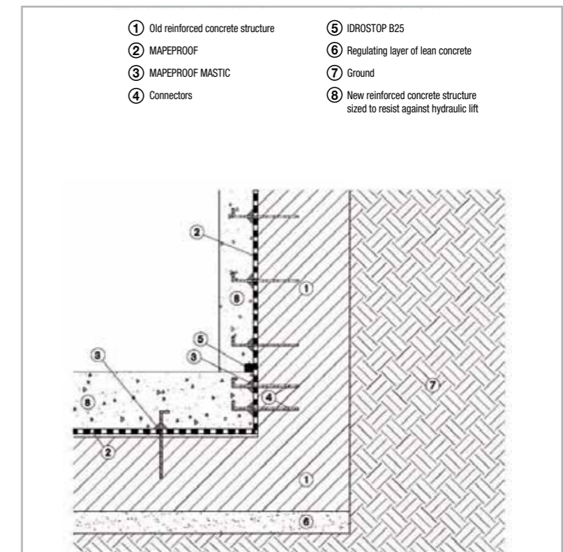
Fig. 8.4 – Detailed layout of relining the inside of a room by applying Mapeproof on the horizontal and vertical surfaces and then casting the reinforced concrete floor slab and retaining walls
