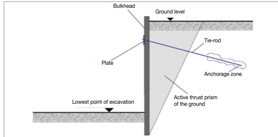
Fig. 4.4 – Anchorage points for stays inserted out of the ground's active thrust zone
