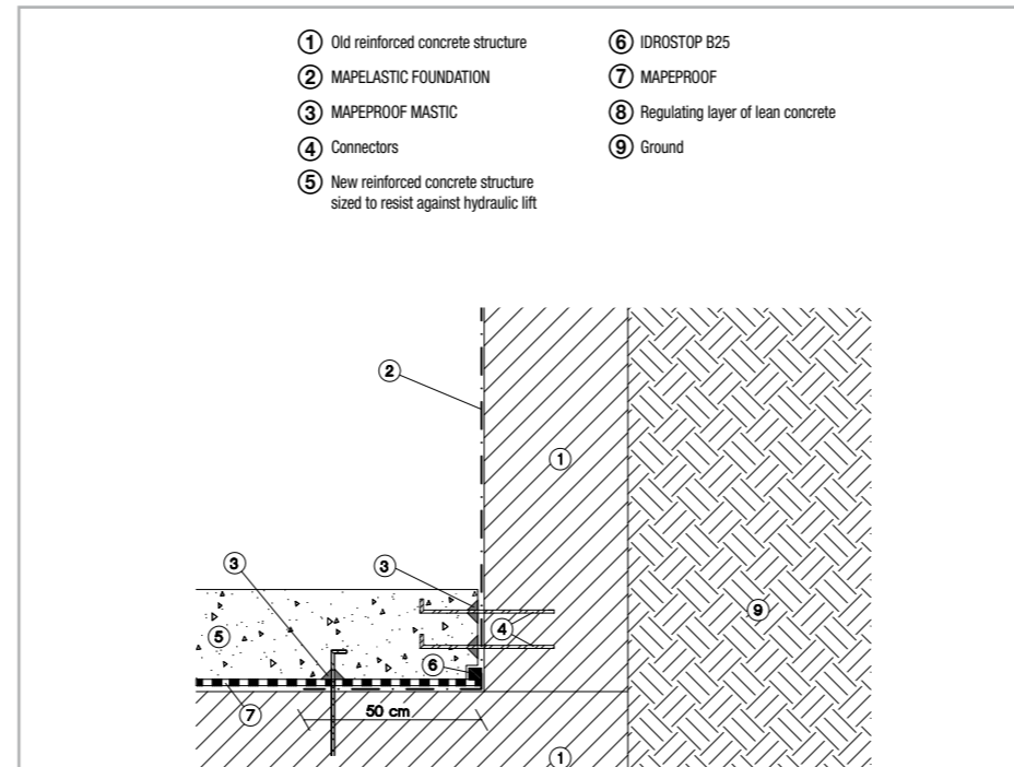
Fig. 8.9 - Detailed layout of relining the inside of a lift well by applying MAPEPROOF on the horizontal surface and MAPELASTIC FOUNDATION on the vertical surface: fillet joint between the floor slab and retaining wall
