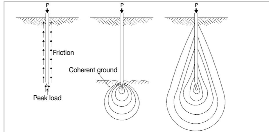
Fig. 2.6 – Schematic diagram of strains acting on a foundation pile
