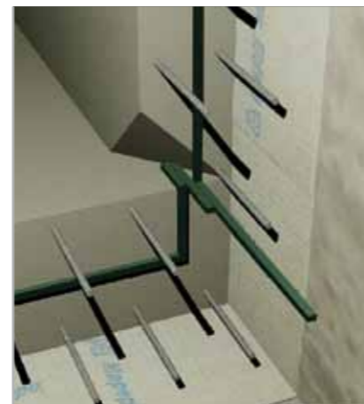
Fig. 7.30 – Strips of IDROSTOP B25 used to seal construction joints in the foundation pad alongside a strip used to seal construction joints between the foundation pad and the walls and between the walls
