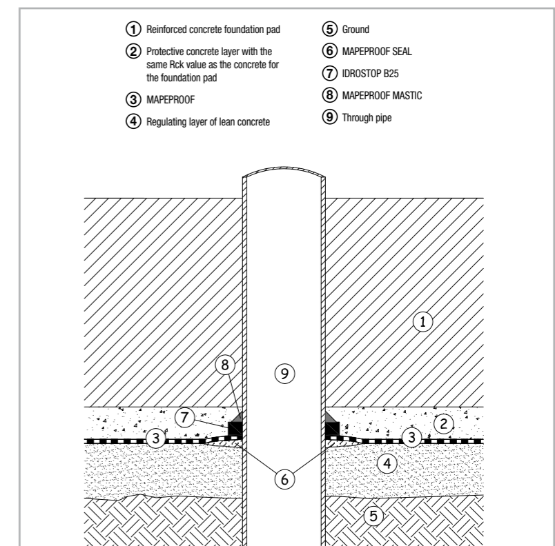
Fig. 7.59 – Detailed layout of sealing a pipe which passes through a foundation pad
