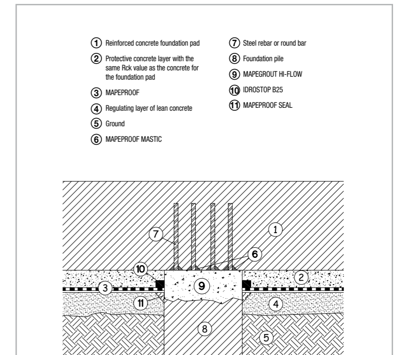
Fig. 7.14 – Detailed layout of waterproofing the heads of piles which work together with the foundation pad and pass through the bentonite sheet
