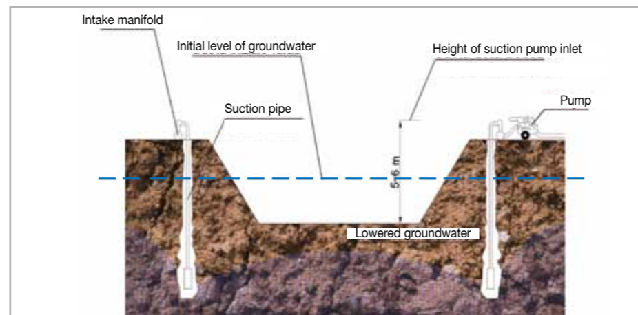
Fig. 3.5 – Schematic diagram of how the level of the water table is lowered using a wellpoint system
