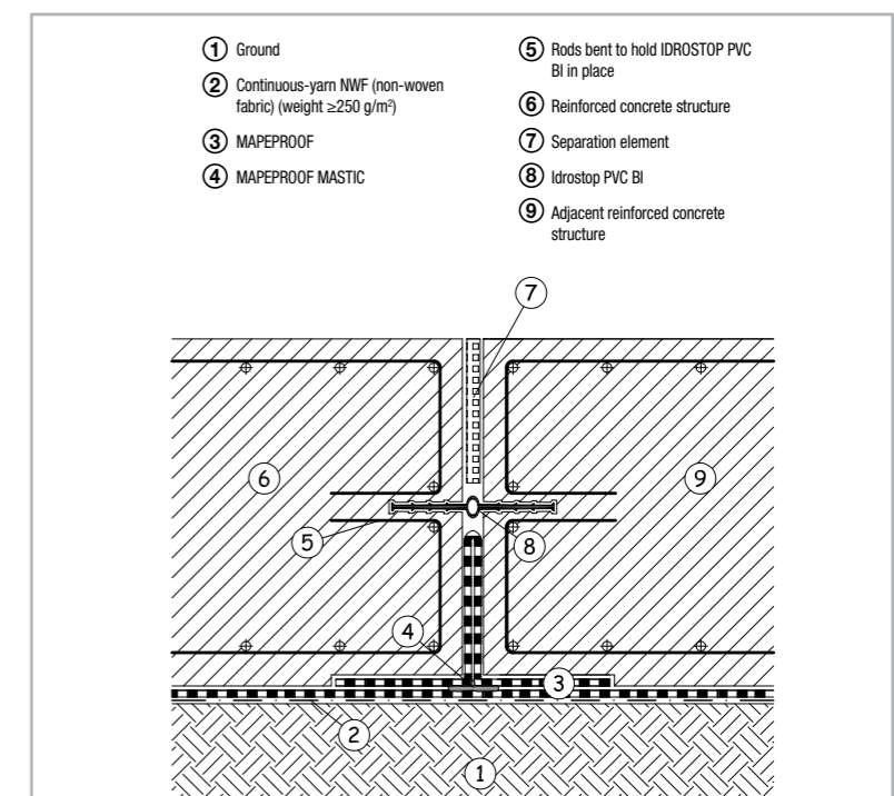
Fig. 7.57 – Detailed layout of sealing a structural joint with IDROSTOP PVC BI
