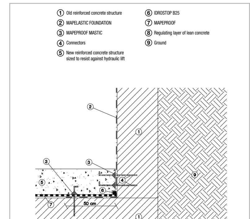
Fig. 8.7a - Detailed layout of relining the inside of a room by applying MAPEPROOF on the horizontal surfaces and MAPELASTIC FOUNDATION on the vertical surfaces: fillet joint between the floor slab and retaining wall
