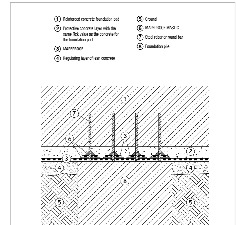
Fig. 7.23 - Detailed layout of waterproofing the heads of piles which work together with the foundation pad without passing through the bentonite sheet
