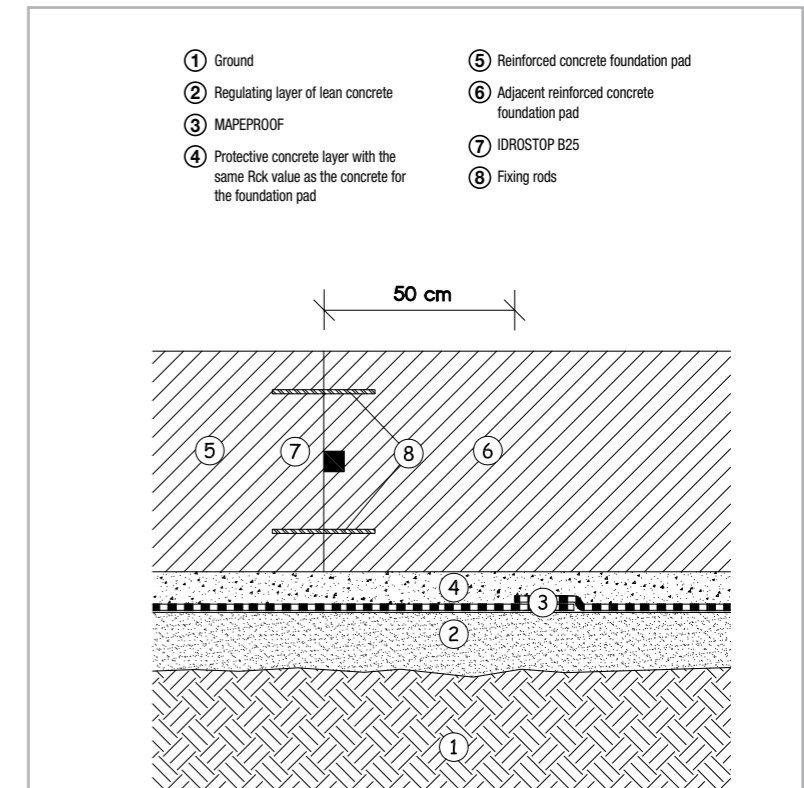
Fig. 7.28 - Detailed layout of sealing a construction joint on a foundation pad
