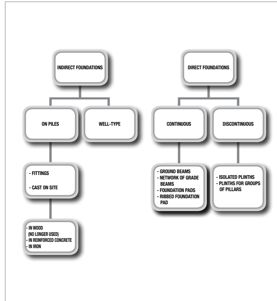
Fig. 2.1 – Classification of foundations according to their load transfer mechanism to the ground
