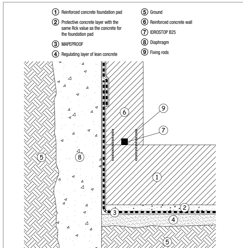
Fig. 7.39 – Detailed layout of applying MAPEPROOF against a diaphragm
