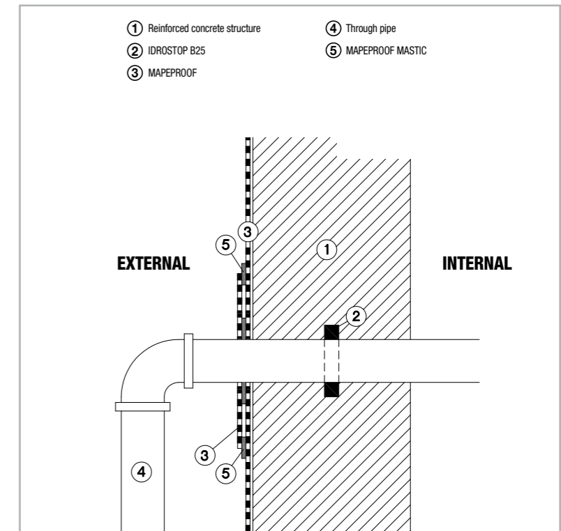
Fig. 7.58 – Detailed layout of sealing a pipe which passes through a facing wall
