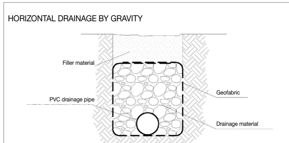
Fig. 3.8 – Schematic view of a horizontal gravitational drainage system, with and without a drainage pipe
