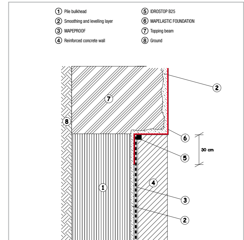
Fig. 7.76 – Waterproofing the topping beam on a bulkhead
