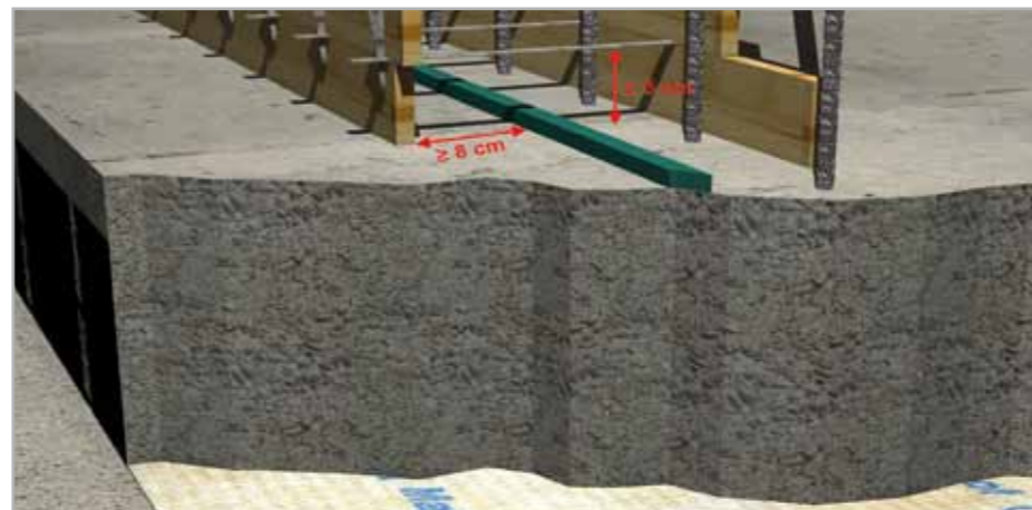
Fig. 7.2 - The minimum distances which must be maintained between IDROSTOP B25 and the blades in formwork, and between IDROSTOP B25 and the outer surface of concrete, to guarantee correct confinement
