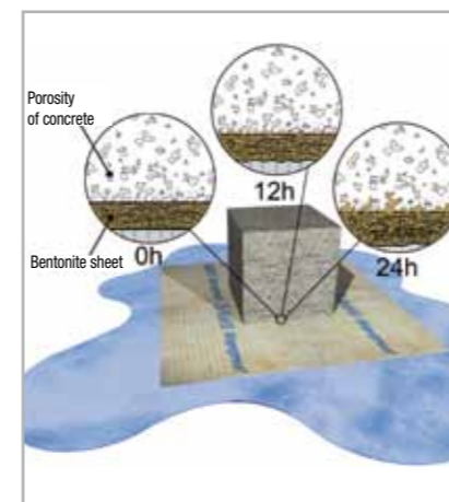
Fig. 5.4 – Hydration process of sodium bentonite contained in MAPEPROOF and MAPEPROOF LW. If the bentonite is confined, when it swells it blocks porosity and impedes the passage of water
