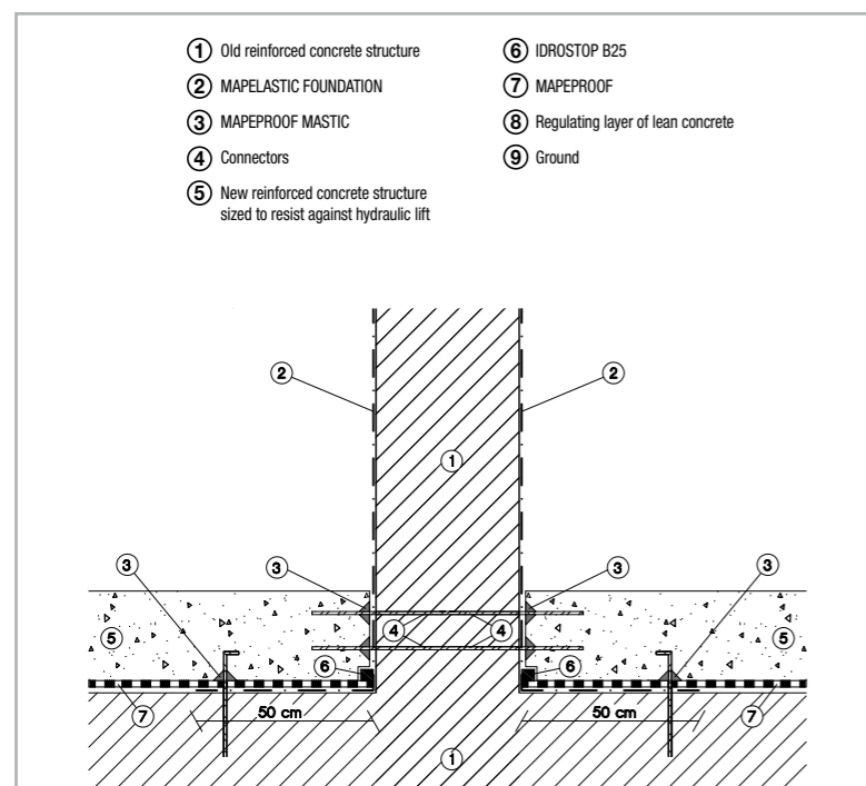
Fig. 8.7b - Detailed layout of relining the inside of a room by applying MAPEPROOF on the horizontal surfaces and MAPELASTIC FOUNDATION on the vertical surfaces: fillet joint between the floor slab and a pillar or parting wall
