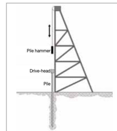
Fig. 2.8 – Schematic diagram of a pile being rammed into the ground
