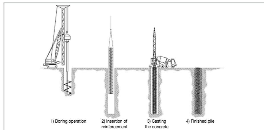
Fig. 2.7 – Phases of the construction of bored piles
