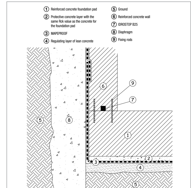
Fig. 7.40 – Detailed layout of applying MAPEPROOF against a diaphragm which works together with the structure
