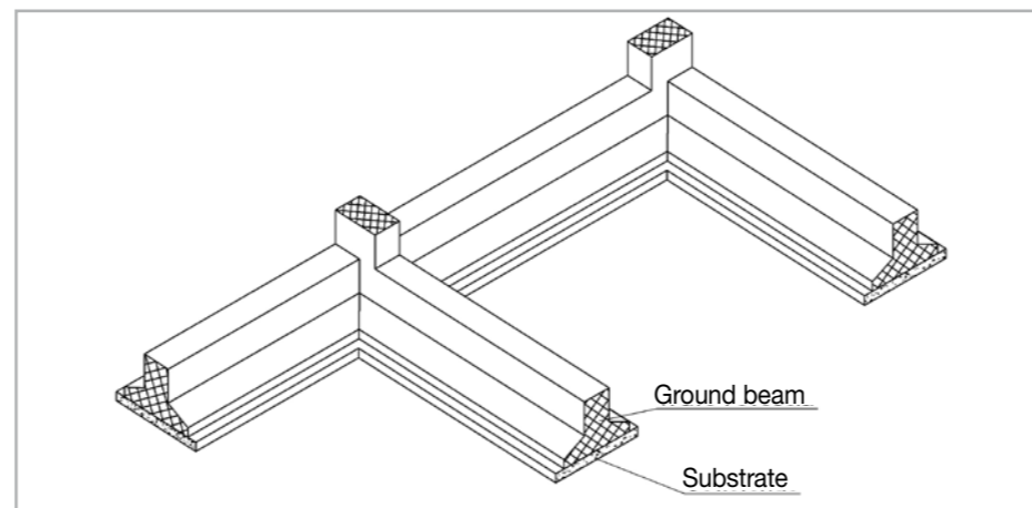
Fig. 2.4 – Lattice of a ground beam
