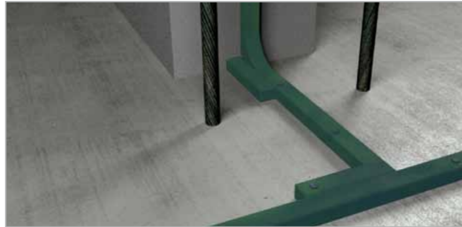
Fig. 7.41 – Strips of IDROSTOP B25 used to seal construction joints between a foundation pad and the walls and construction joints between adjacent walls
