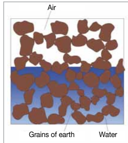
Fig. 3.1 - Schematic sectional view of a portion of ground
