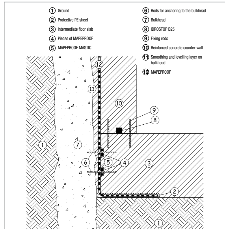
Fig. 7.65 – Detailed layout of waterproofing the end of an intermediate floor slab in a top-down construction
