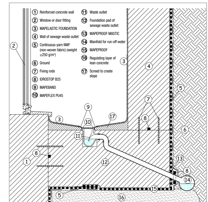
Fig. 7.64 - Detailed layout of waterproofing an aeration outlet cast in place
