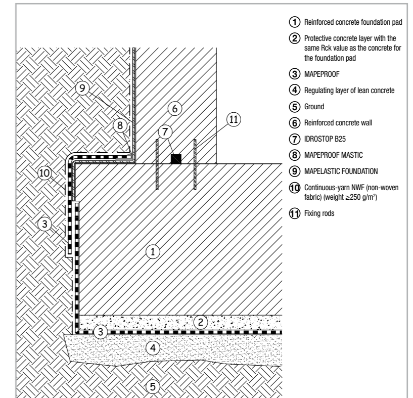
Fig. 7.46 – Detailed layout of waterproofing a foundation pad with MAPEPROOF and MAPELASTIC FOUNDATION applied on the wall
