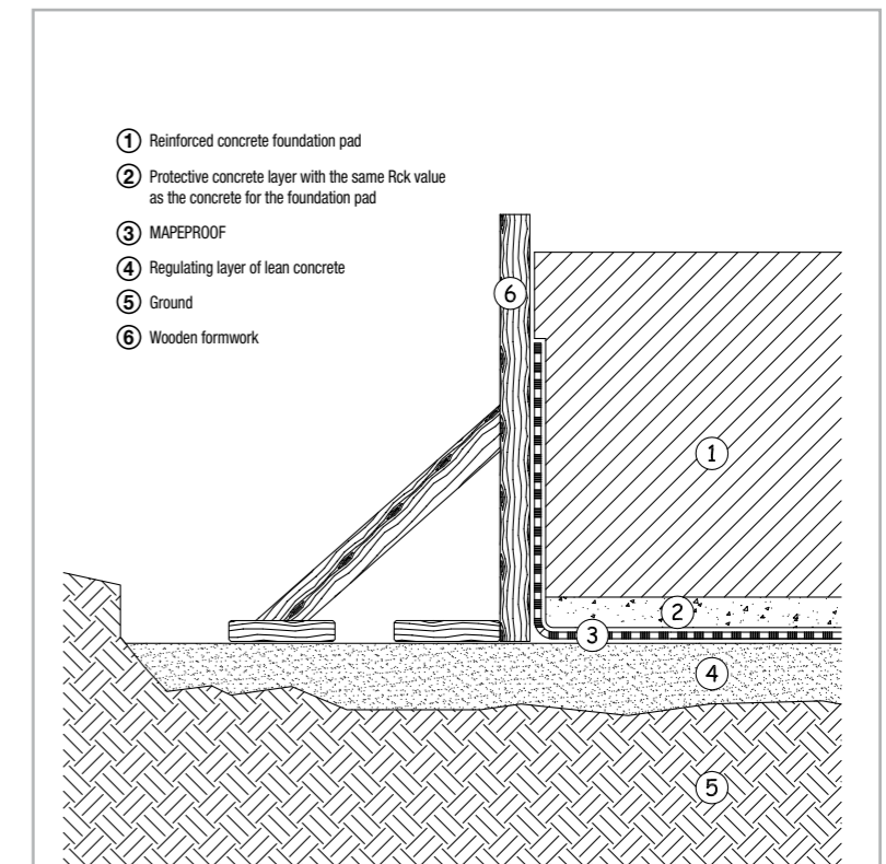
Fig. 7.8 – Detailed layout of MAPEPROOF applied on wooden formwork
