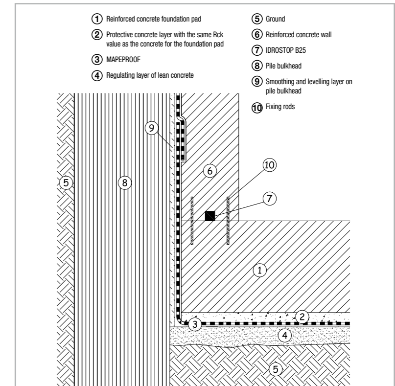
Fig. 7.34 – Detailed layout of applying Mapeproof against a pile bulwark with a surface which has been levelled off
