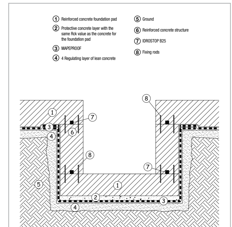
Fig. 7.6 – Detailed layout of waterproofing a lift well
