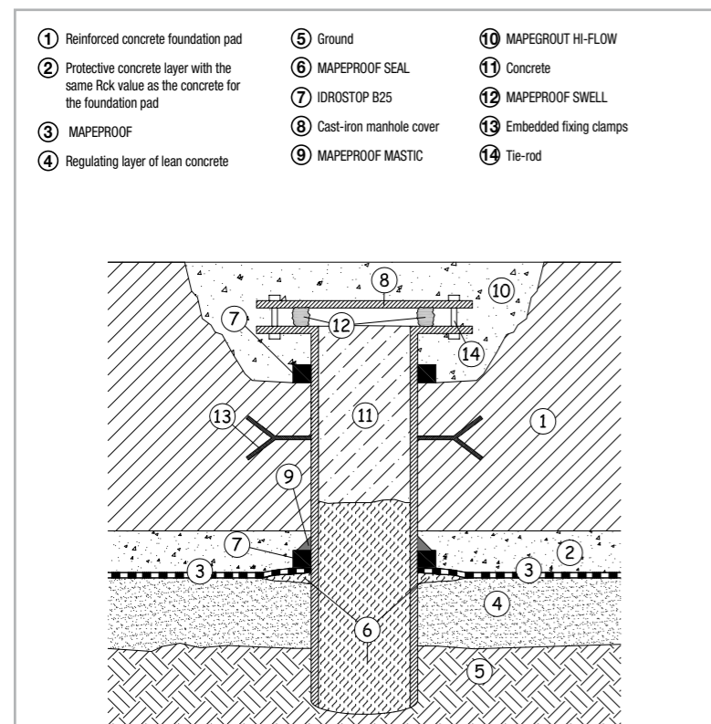
Fig. 7.62 – Detailed layout of sealing a drainage well embedded in the foundation pad
