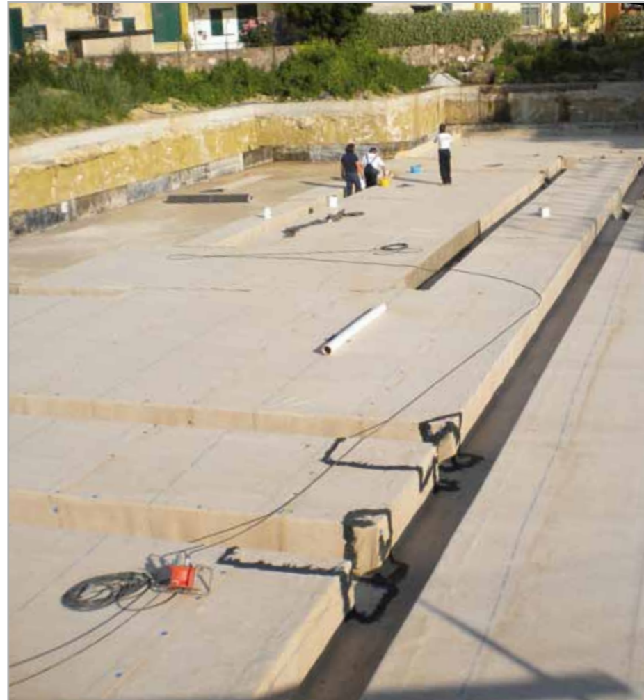
Fig. 7.11 – Waterproofing a ribbed foundation pad by applying MAPEPROOF
