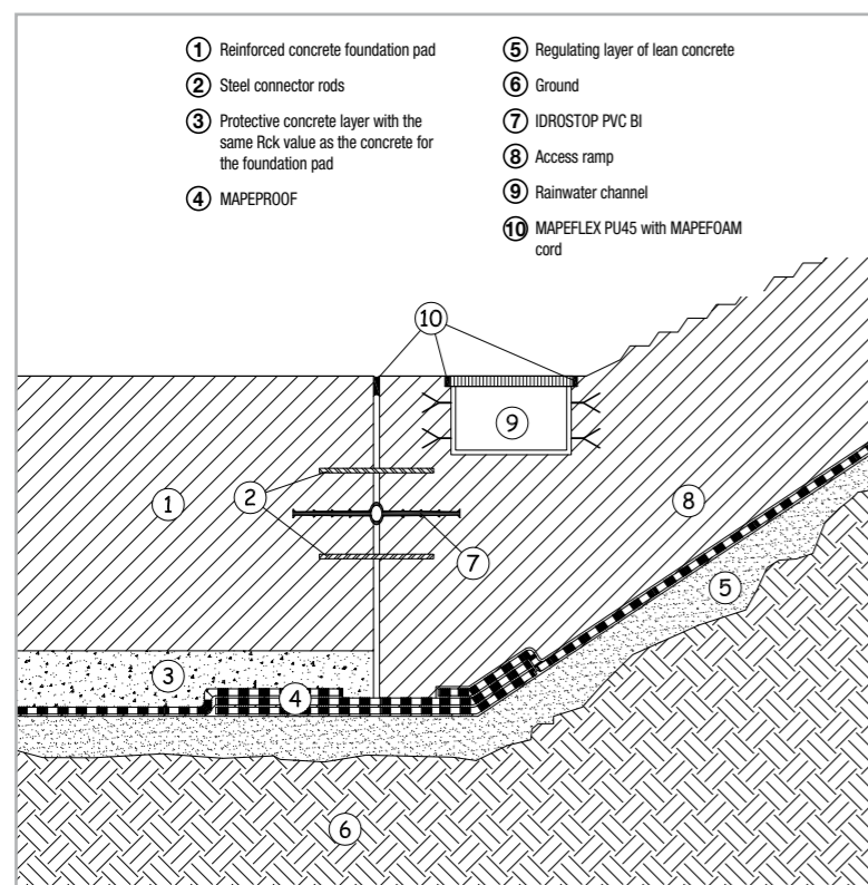
Fig. 7.63 - Detailed layout of waterproofing an access ramp to an underground garage which is structurally independent from the rest of the building
