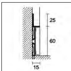
88/6 + 88/16SF Einsatz in Aluminium
