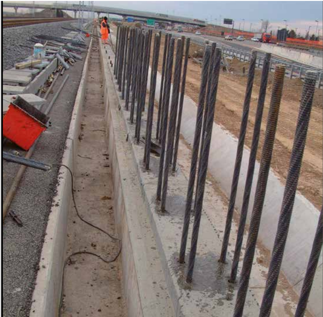
Photo 12 Anchoring steel bars in concrete using PLANIGROUT 300
